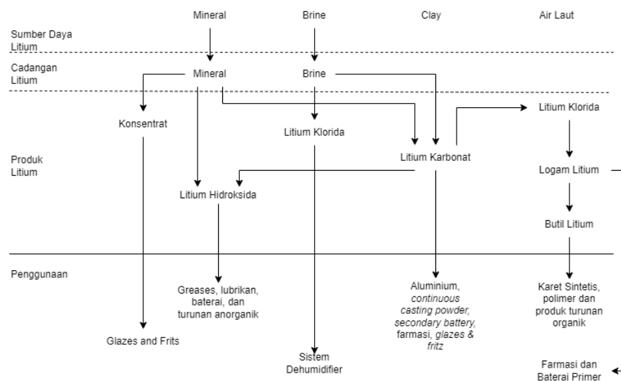
Figure 5 Lithium Processing Industrial Tree
