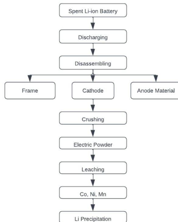
Figure 2 Lithium-Ion Battery Hydrometallurgy Process
