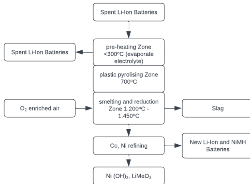
Figure 3 Lithium-Ion Battery Pyrometallurgy Process
